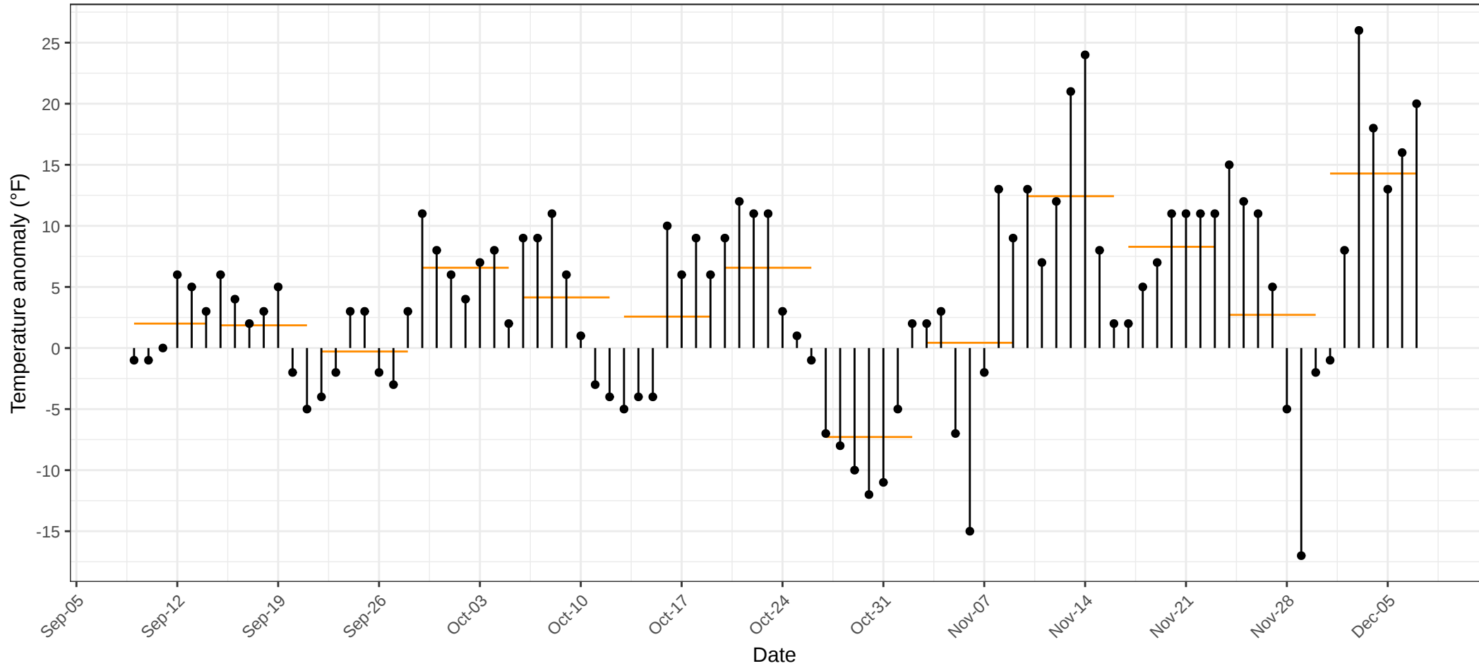
Difference between daily mean temperature and 30-year average, Fairbanks Airport (PAFA) 2022
