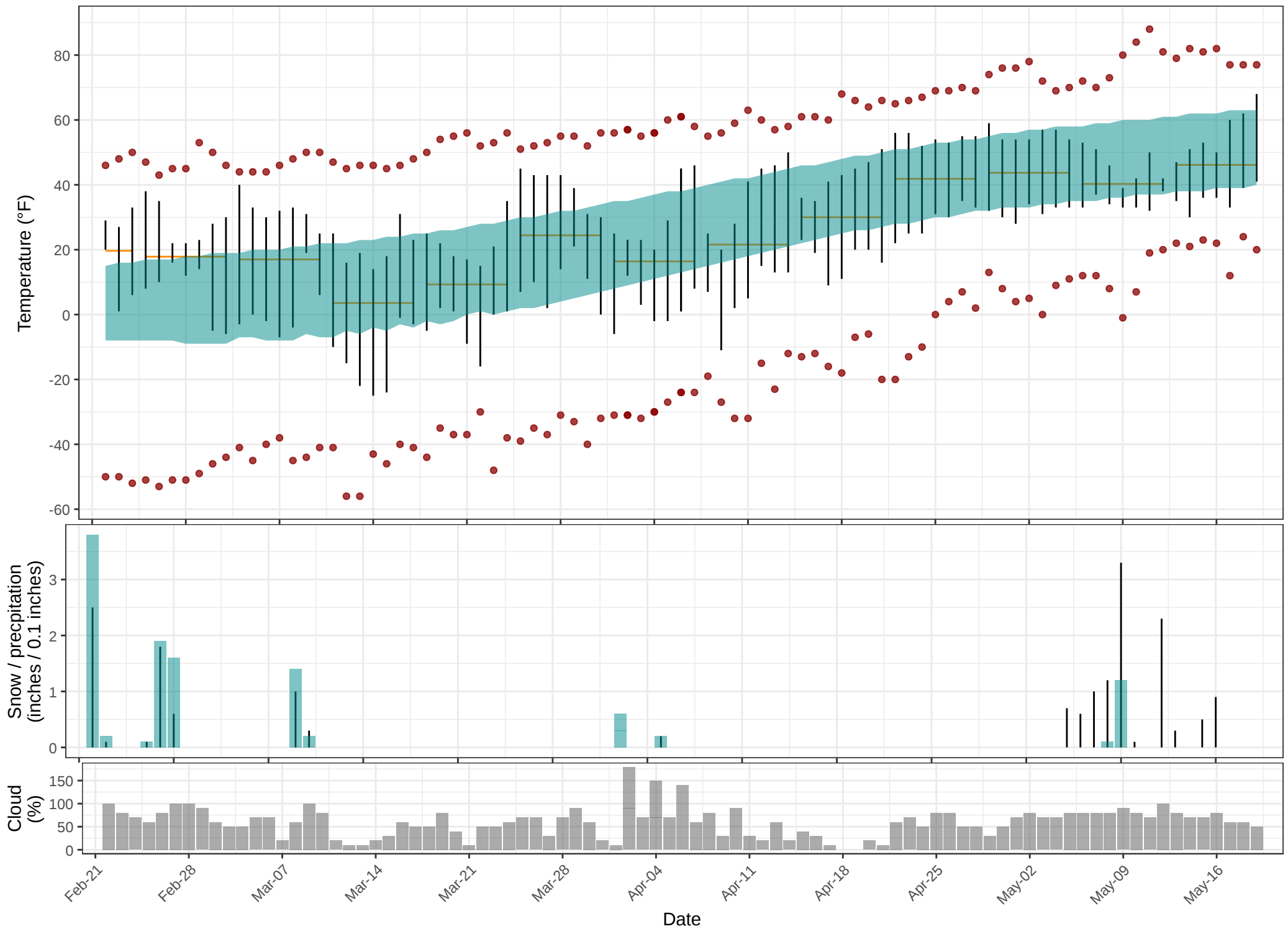
Daily temperature, precipitation and cloud cover, Fairbanks Airport (PAFA) 2022
