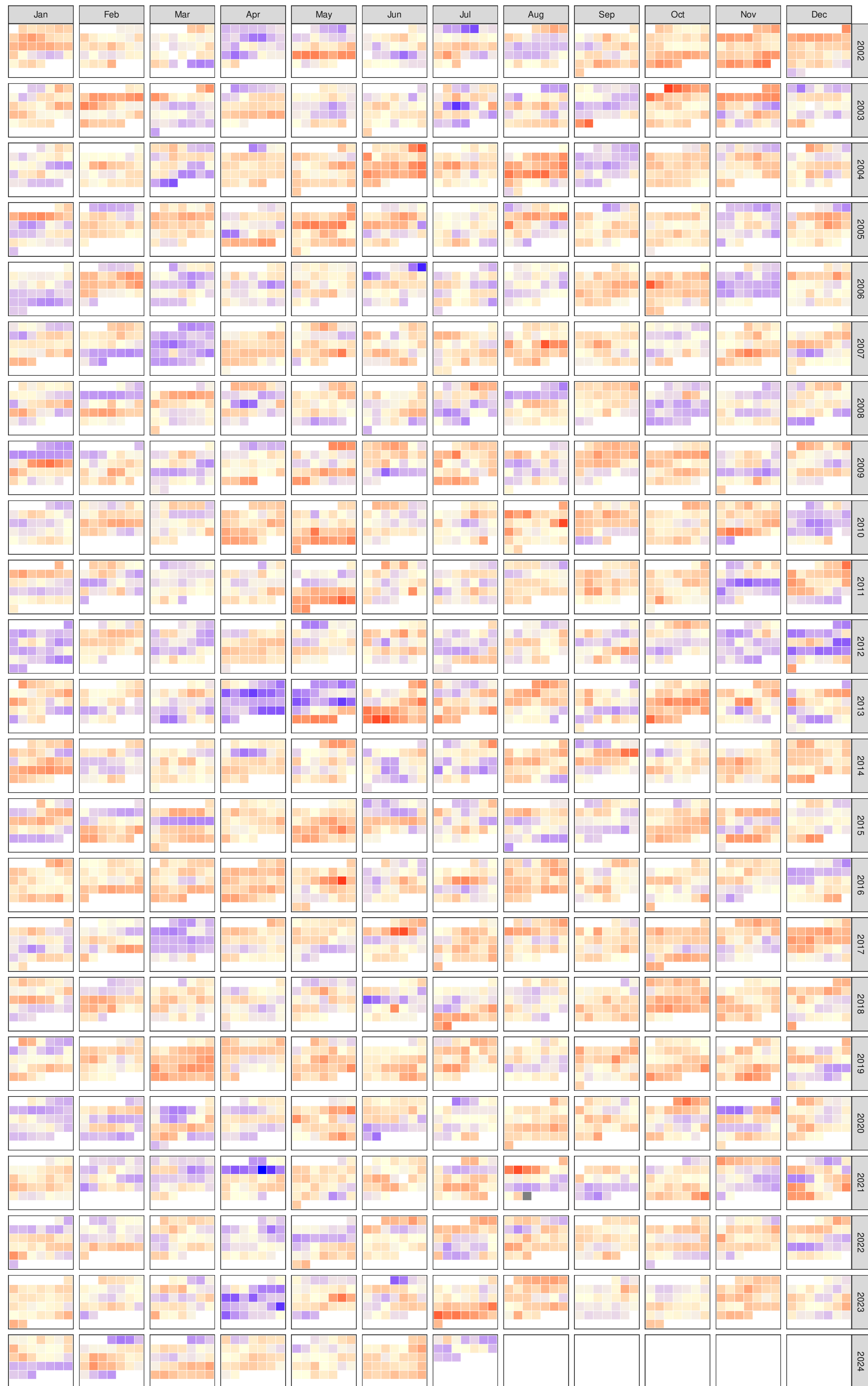
Normalized difference between daily mean temperature and 30-year average
